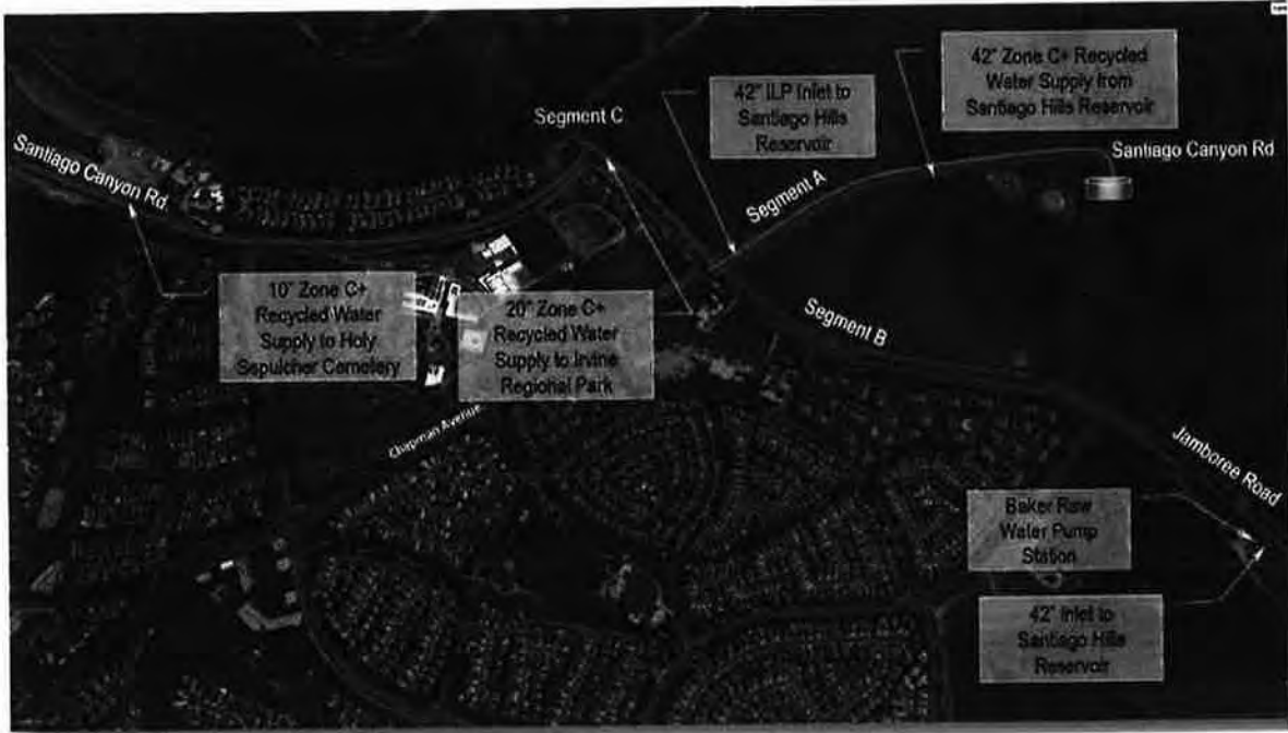
42-Inch Irvine Lake Inlet Pipeline to Santiago Hills Reservoir, 42-Inch Zone C+ Recycled Water Supply Pipeline from Santiago Hills Reservoir, and 20-inch Zone C+ Recycled Water Supply Pipeline to Irvine Regional Park
